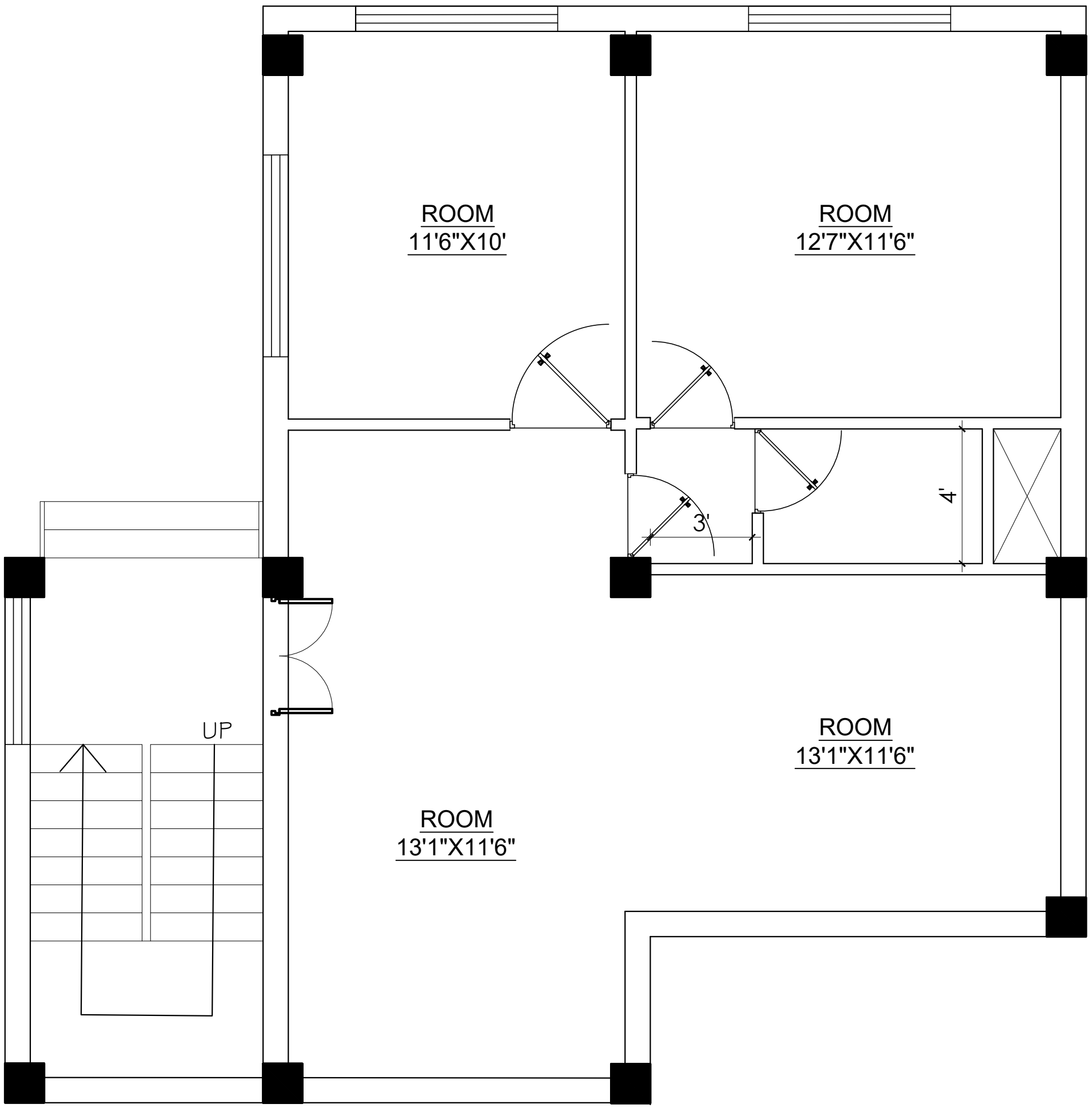
GROUND FLOOR PLAN AREA : 856.5 SQ.FT.
